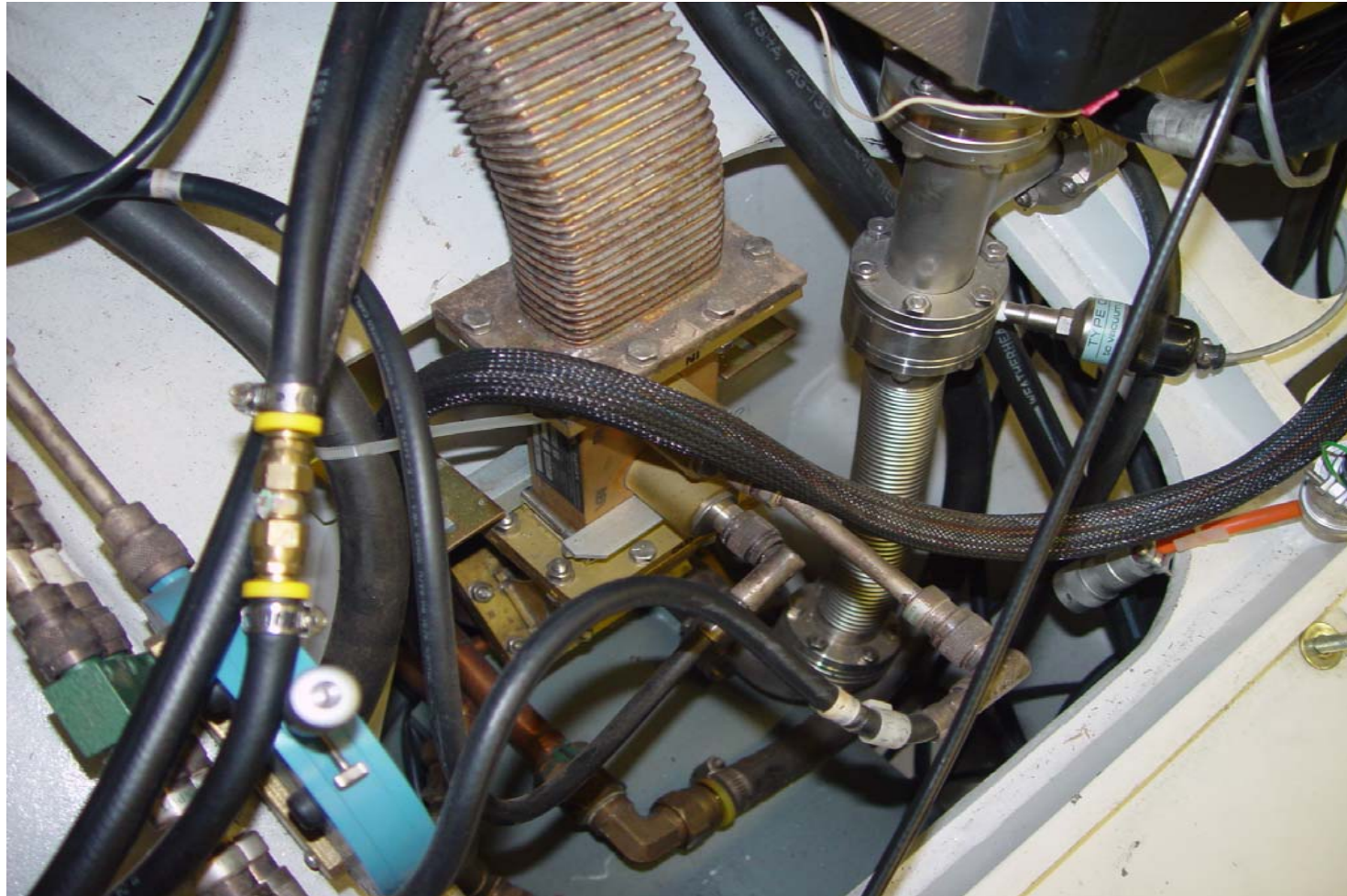
Waveguide Connection to Accelerator (from top)
